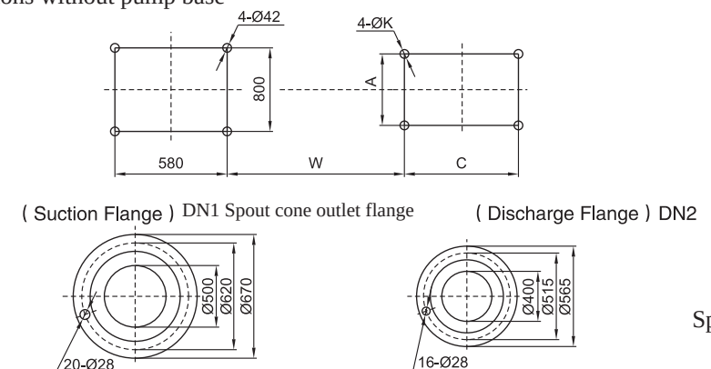
Mounting base dimensions without pump base
