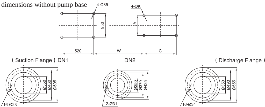
Spout cone length E=300
