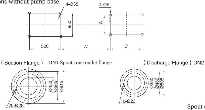
Mounting base dimensions without pump base
