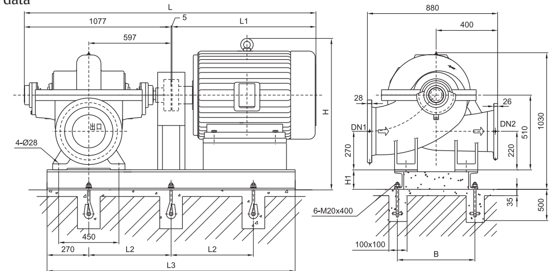
Mounting base dimensions without pump base
