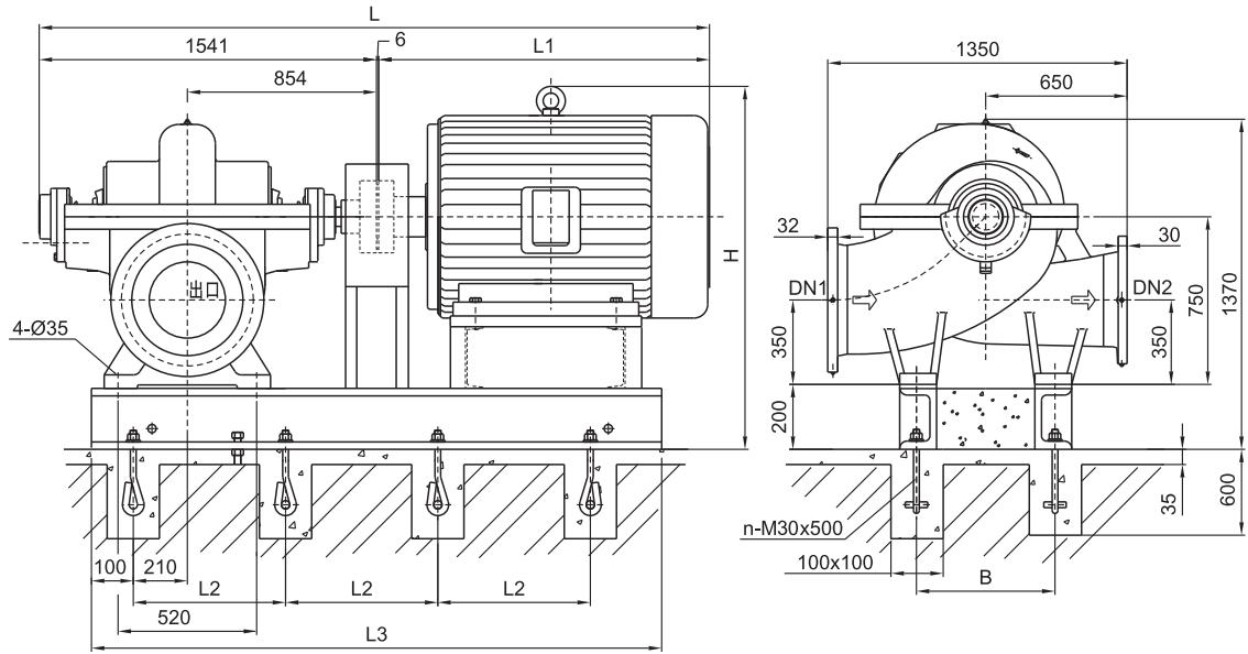
Mounting base dimensions without pump base
