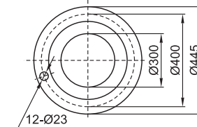
( Suction Flange ) DN1 Spout cone outlet flange
