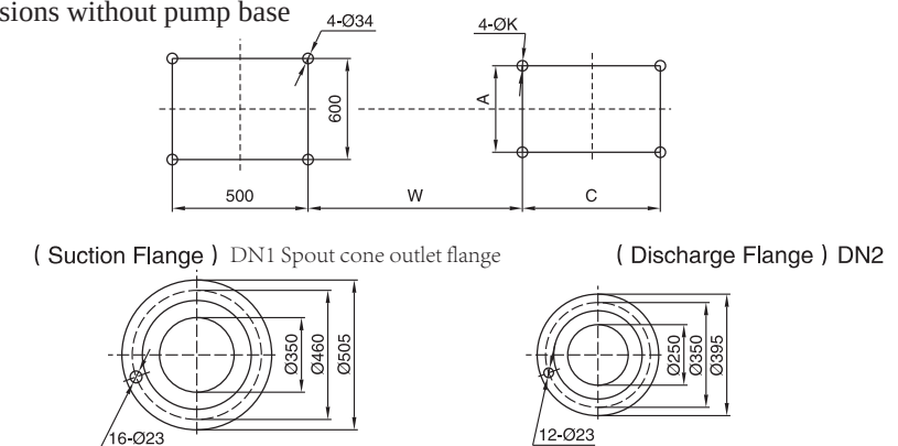
Mounting base dimensions without pump base
