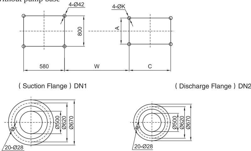
Mounting base dimensions without pump base
