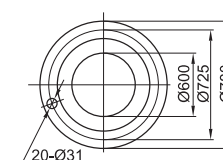
( Suction Flange ) DN1
