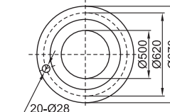
( Suction Flange ) DN1 Spout cone outlet flange
