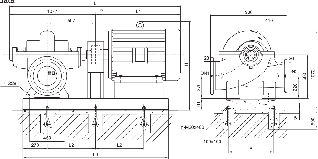
Mounting base dimensions without pump base
