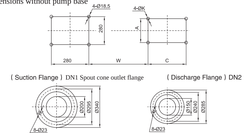
Mounting base dimensions without pump base
