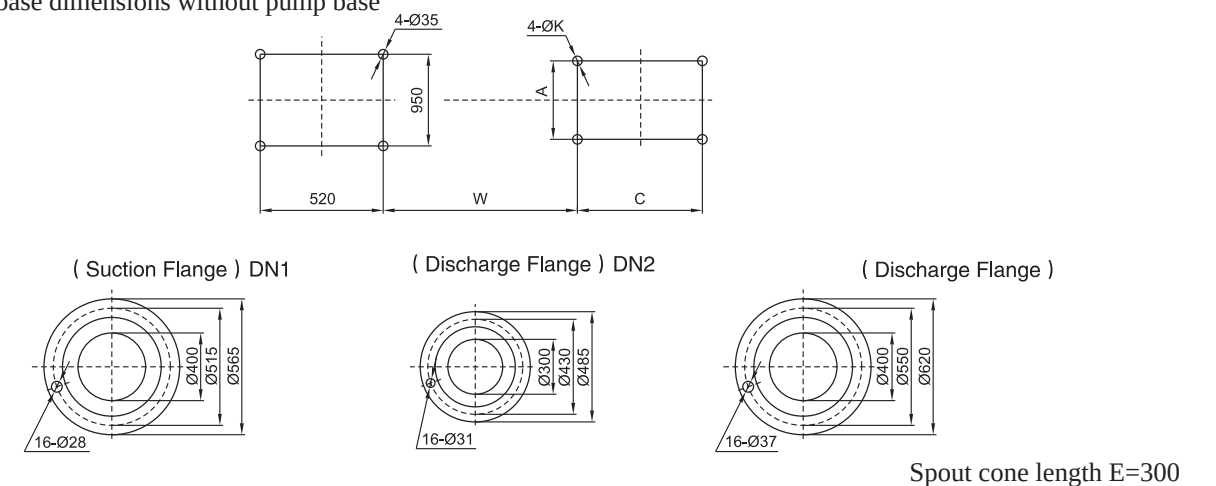
Mounting base dimensions without pump base
