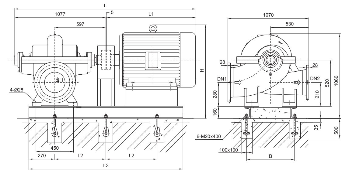
Mounting base dimensions without pump base
