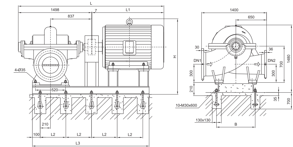
Mounting base dimensions without pump base
