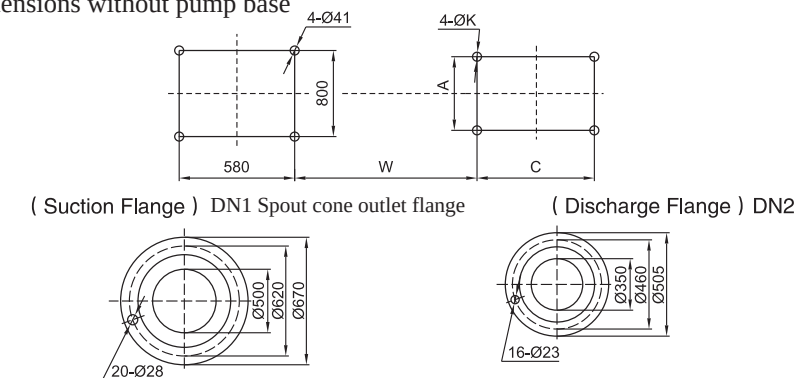
Mounting base dimensions without pump base
