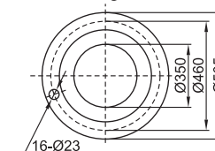
( Suction Flange ) DN1 Spout cone outlet flange
