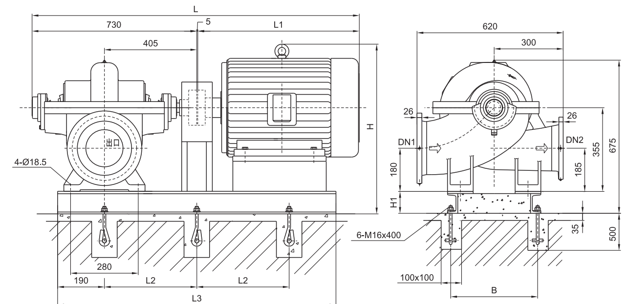
( Suction Flange ) DN1 Spout cone outlet flange
