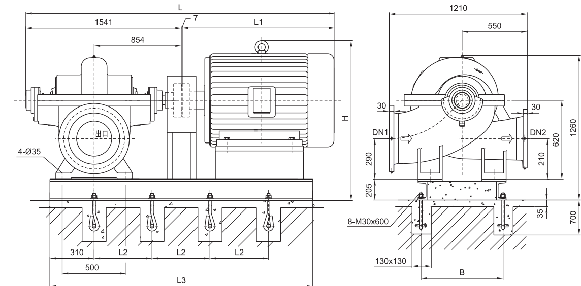
Mounting base dimensions without pump base
