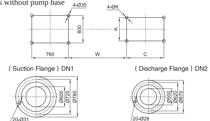
Mounting base dimensions without pump base
