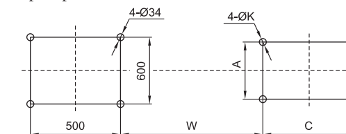
Mounting base dimensions without pump base
