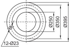
( Suction Flange ) DN1 Spout cone outlet flange
