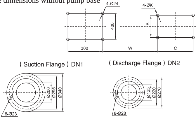
Mounting base dimensions without pump base
