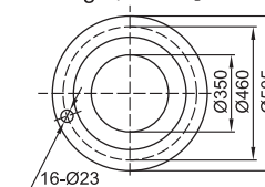
( Suction Flange ) DN1 Spout cone outlet flange
