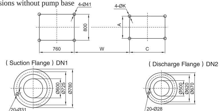
Mounting base dimensions without pump base
