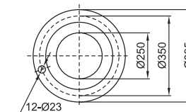
( Suction Flange ) DN1 Spout cone outlet flange
